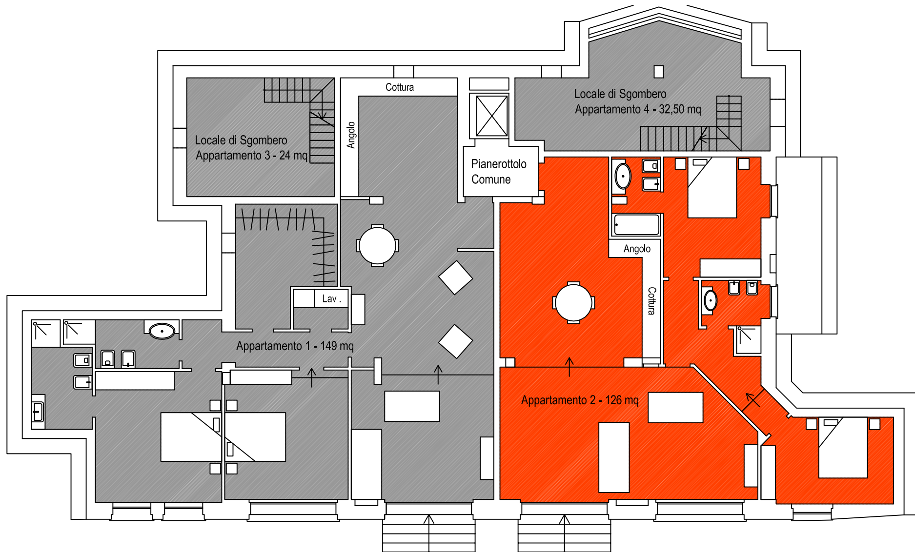
Piano Semi - interrato
